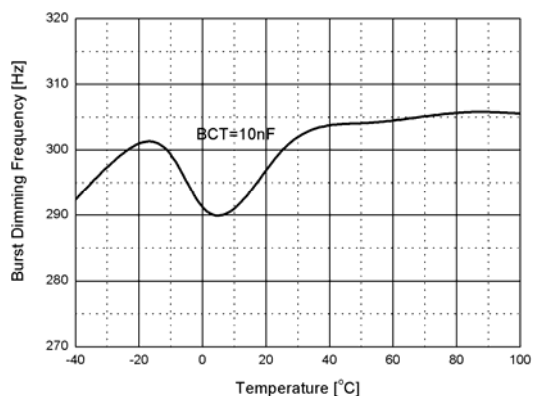
Figure 9. Burst Dimming Frequency vs. Temp.
