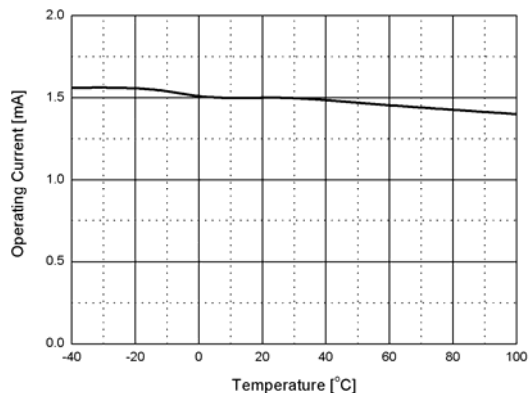
Figure 16. Operating Current vs. Temp.
