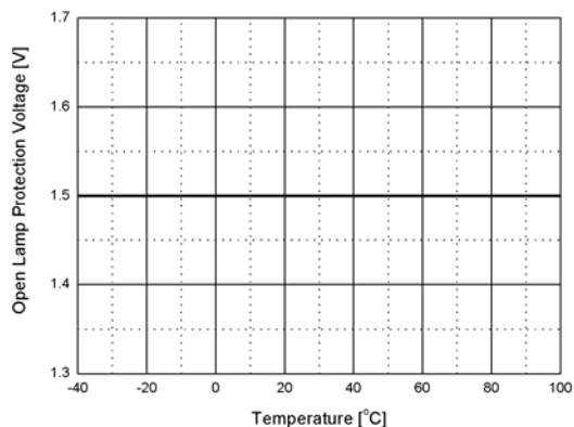
Figure 18. Open-Lamp Protection Voltage vs. Temp.
