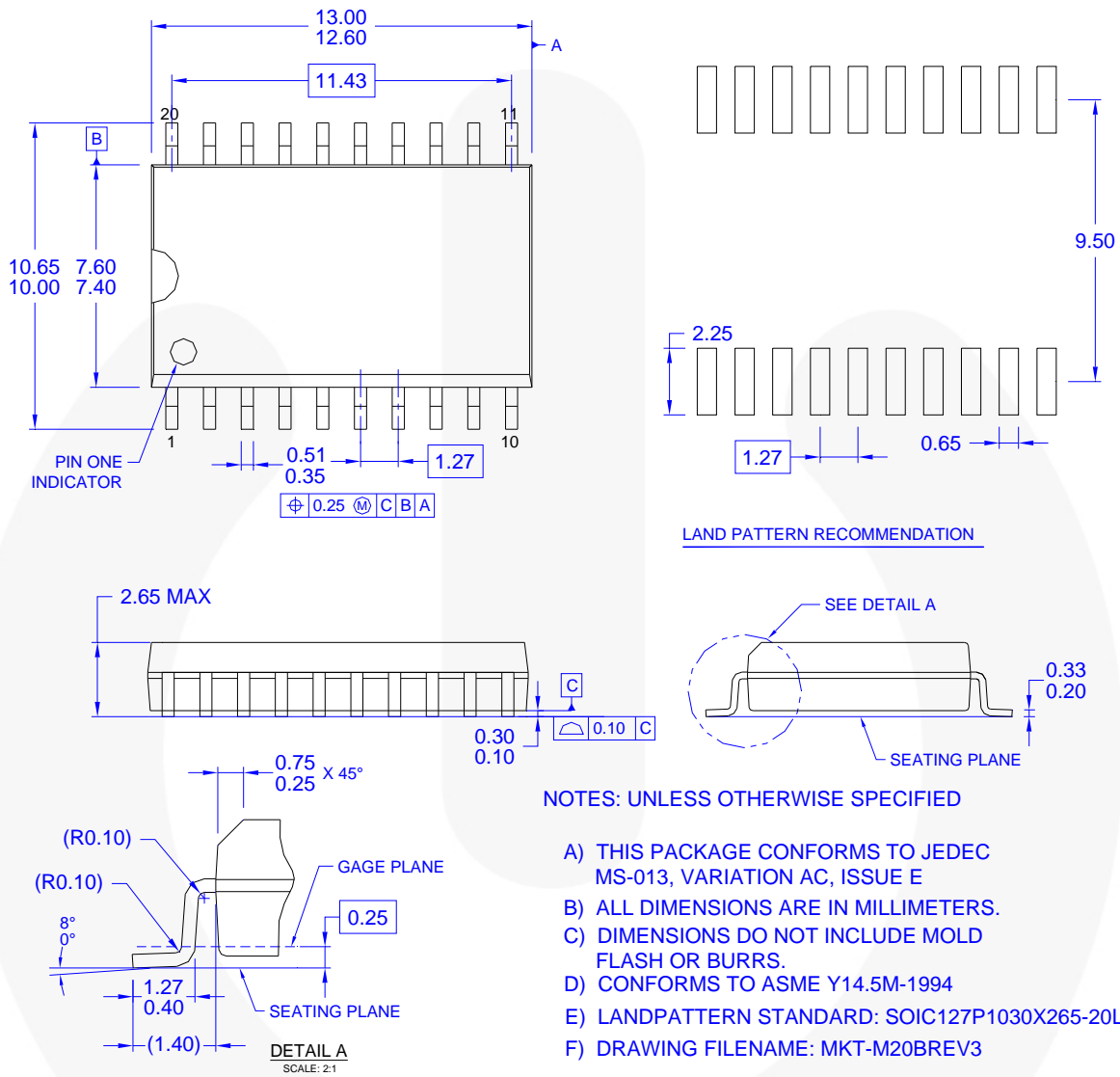
Figure 49. 20-SOIC Package
