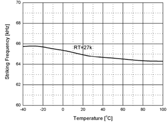
Figure 8. Striking Frequency vs. Temp.
