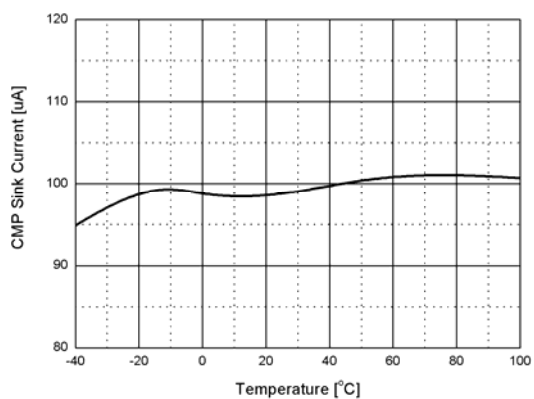
Figure 13. CMP Sink Current vs. Temp.
