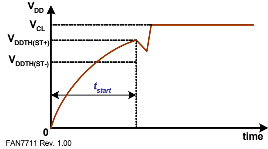
Figure 27. V_{DD} Build-up
